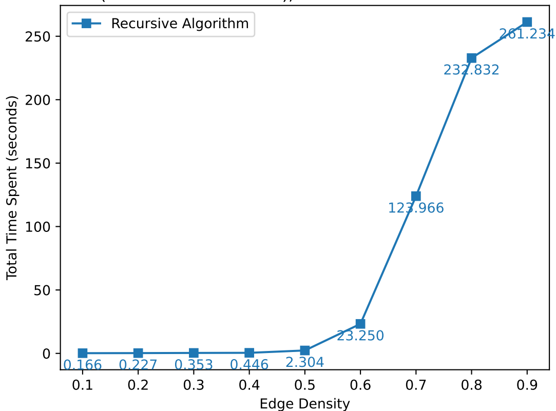
Overall Time Spent on Recursive Algorithm at Different Edge Densities (200 realizations each), basis calculation disabled
